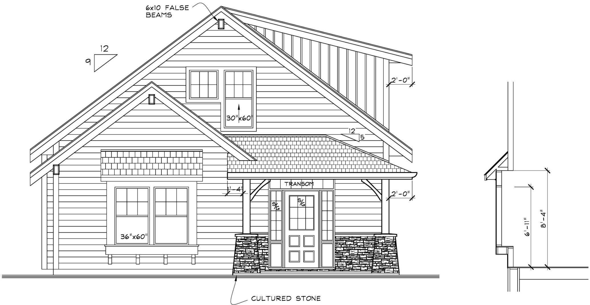
FRONT ELEVATION #2
