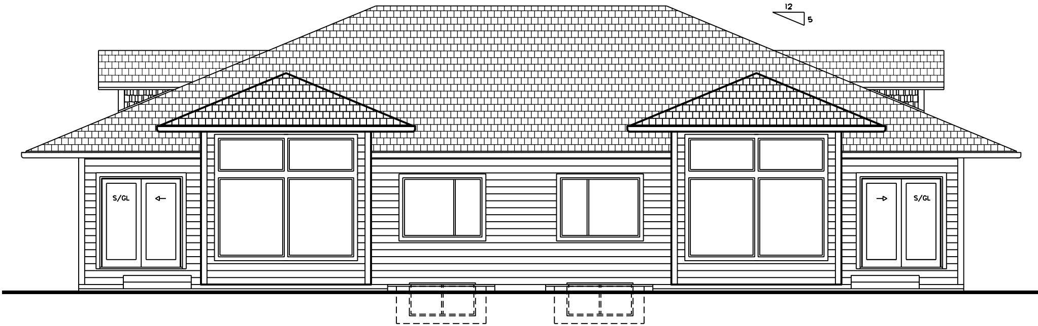
REAR ELEVATION
